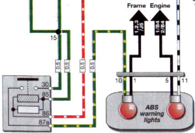
ABS warning relay
